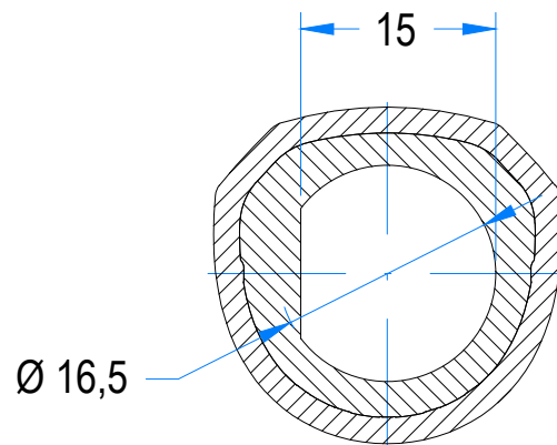
B-B Section
